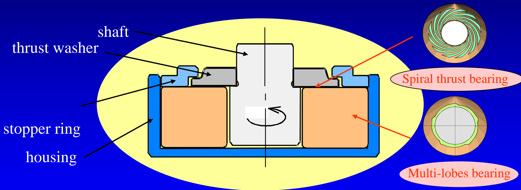
Structure of HMF bearing unit
